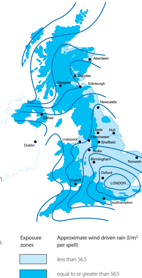
Figure 1: Categories of exposure to driving rain (from BS 5534:2003)
