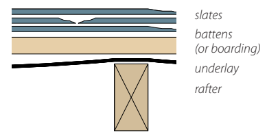
Figure 2: section through typical cold roof construction with slates
