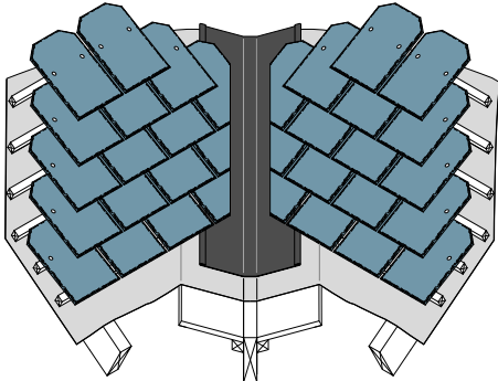
Open valleys
