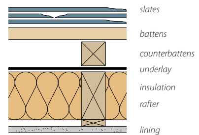
Figure 4: insulation between rafters (full fill)
