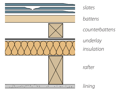
Figure 3: insulation above rafters
