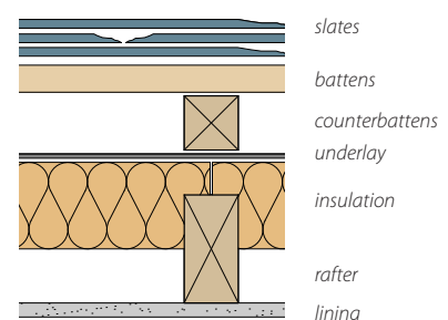
Figure 6: insulation above and between rafters
