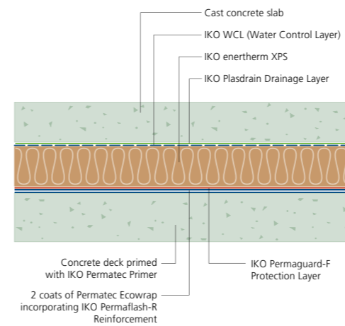
Typical floating concrete base
