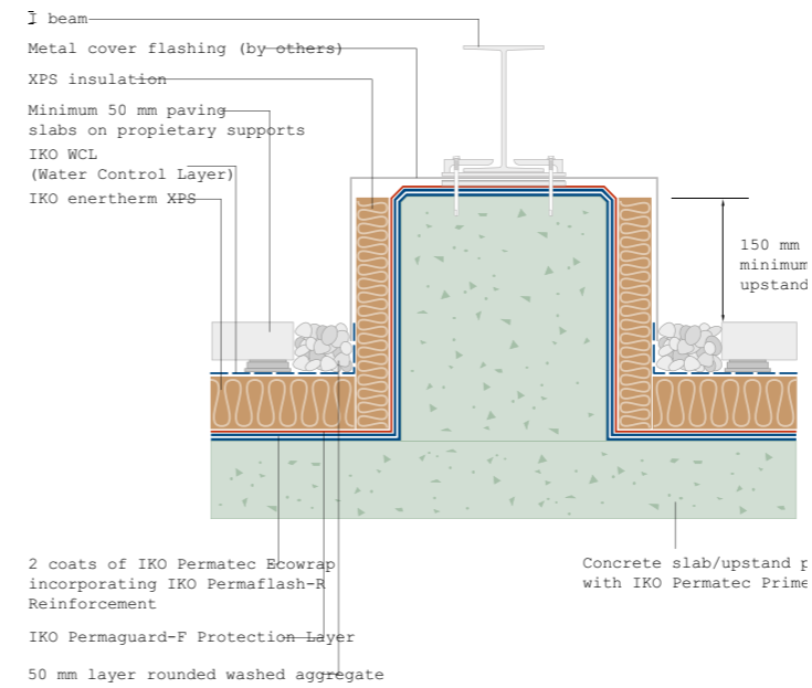
Typical plinth detail
