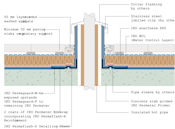
Typical hot pipe detail
