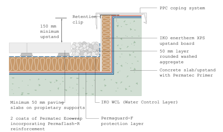
Typical parapet with coping detail
