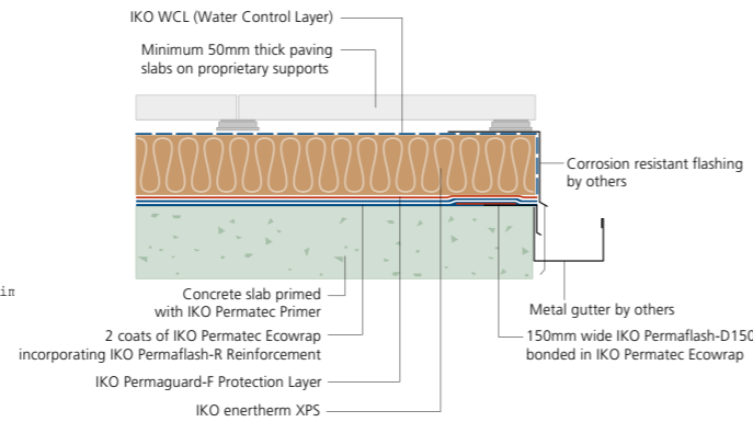
Typical drip to external gutter
