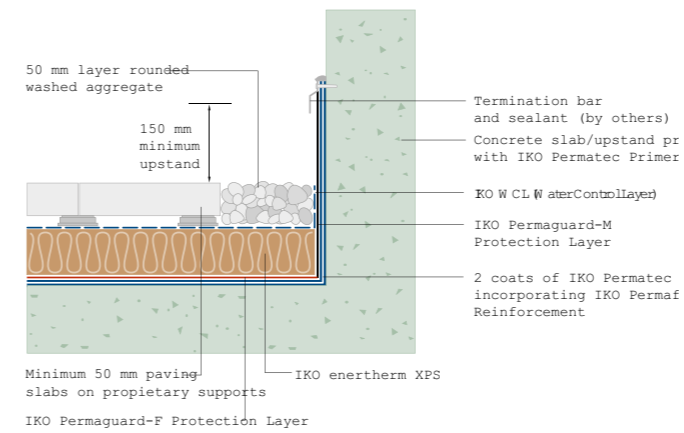
Typical uninsulated upstand with termination detail
