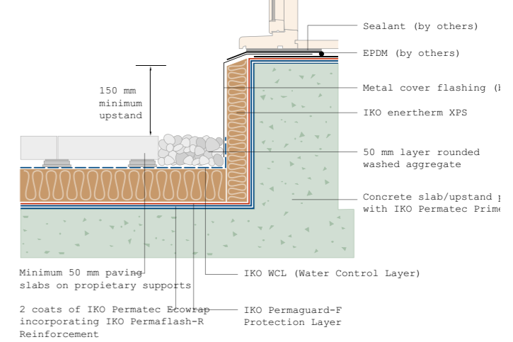
Typical cill section detail
