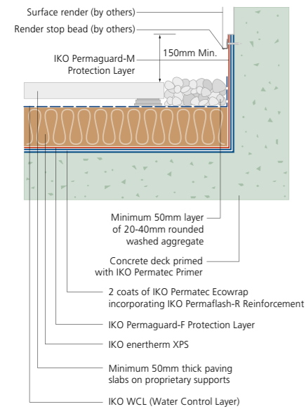
Typical rendered upstand section
