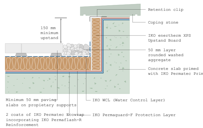
Typical parapet with capping detail
