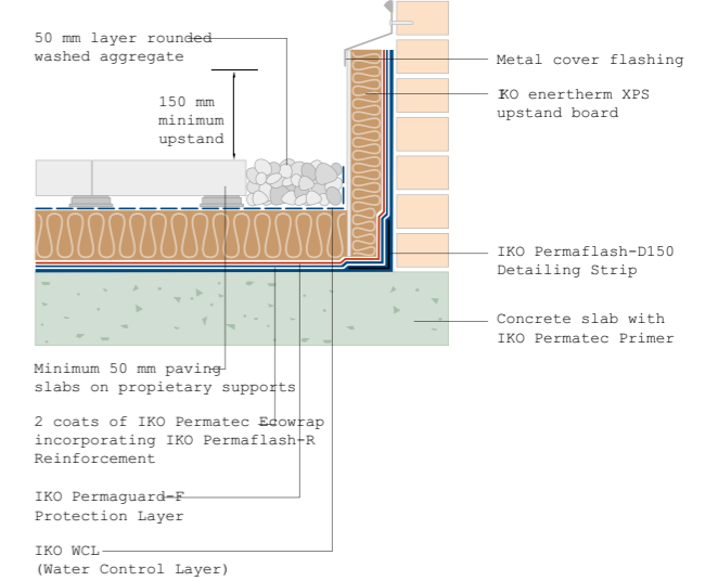
Typical insulated upstand section
