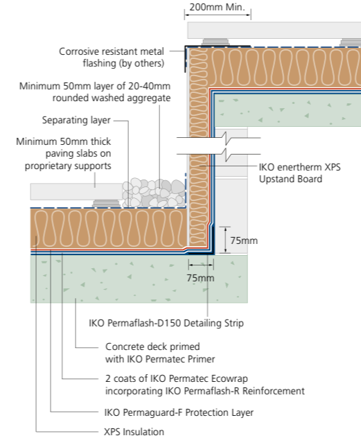
Typical insulated change in level
