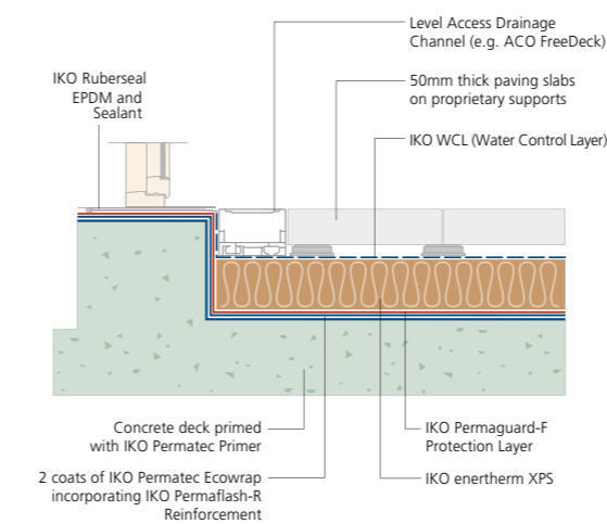
Typical level access threshold
