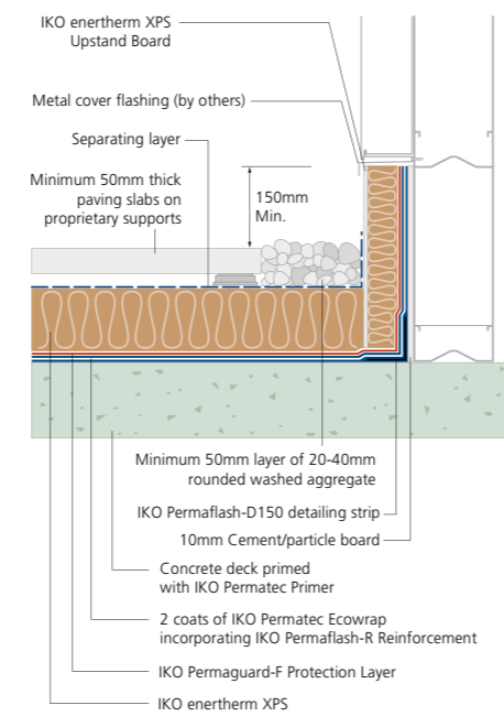
Typical upstand to Metsec
