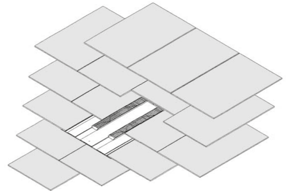
Adjacent slates overlap ventilator outer flanges
