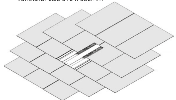
Adjacent slates abut ventilator
