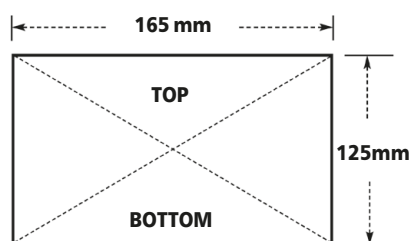
FIG. 3. Roof underlay cutting/folding for soil pipe adapter
