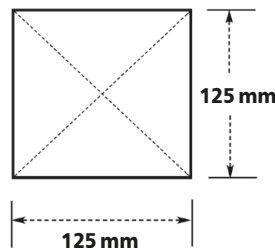
FIG. 3. Roof underlay cutting/folding for soil pipe adapter
