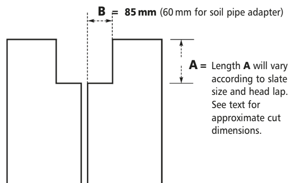
FIG. 2. Roof underlay cutting and folds to achieve full 20,000 mm 2 through flow of air
