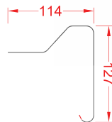
B260 STANDARD RAISED EDGE TRIM
