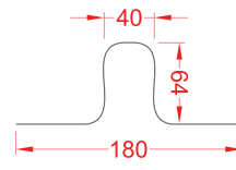
E280 EXPANSION JOINT / ROLL MOP TRIM
