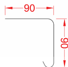
A200 STANDARD DRIP TRIM
